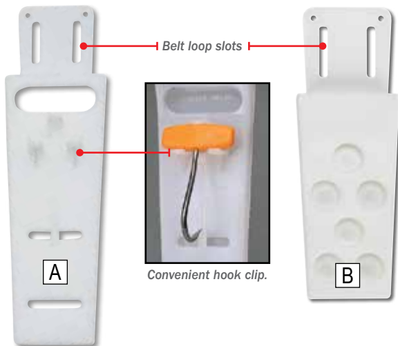
Angled flange keeps knives nestled close to scabbard and safely out of the way.
