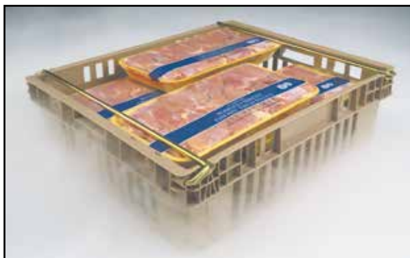
Two 3/8 inch zinc-plated steel wire bails swing down to allow nesting and swing up for stacking.
