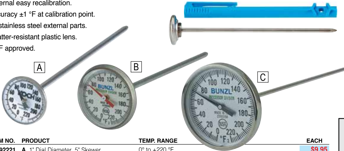
1-inch dial includes probe sheath and pocket clip. FREE Calibration tool included on sheath.
